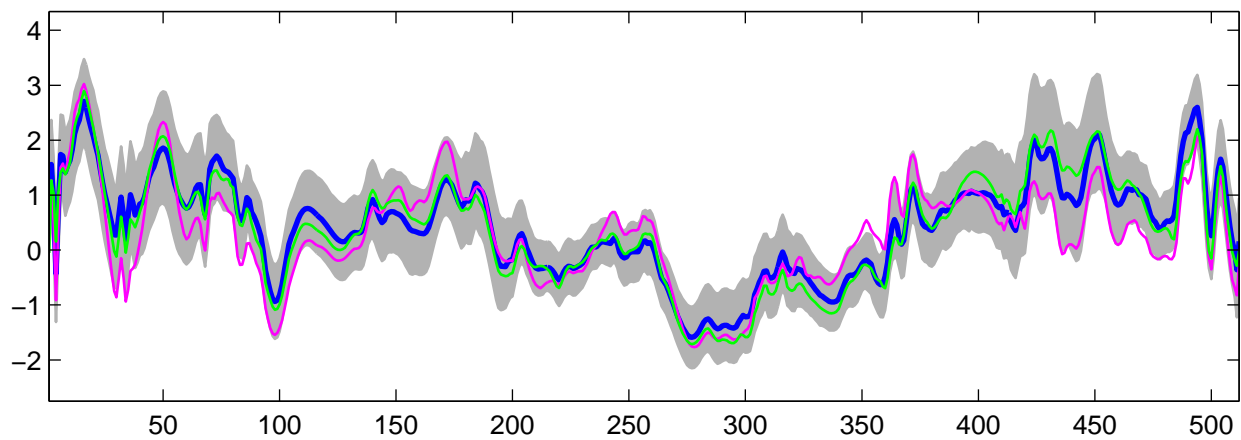
Estimated U_{31}(t) using R-WFMM: Normal data, run 6
