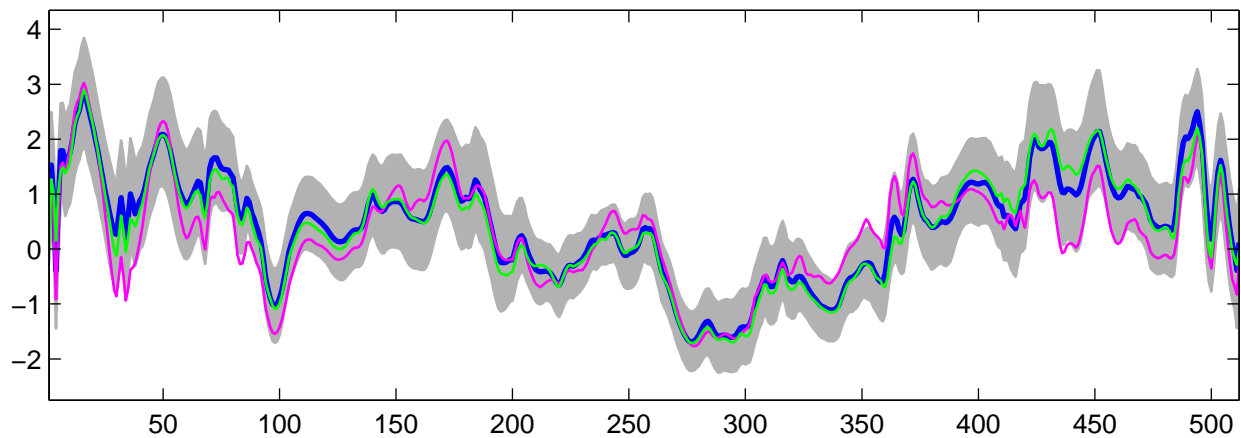
Estimated U_{31}(t) using G-WFMM: Normal data, run 6
