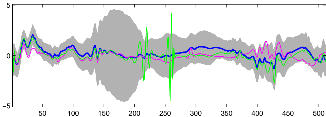
Estimated U_{31}(t) using G-WFMM: t_1 data, run 6
