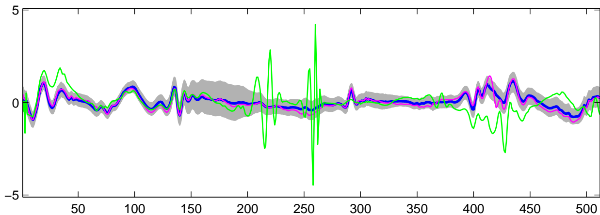
Estimated U_{31}(t) using R-WFMM: t_1 data, run 6
