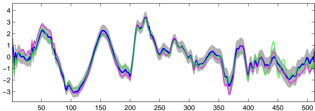
Estimated U_{31}(t) using R-WFMM: t_2 data, run 6
