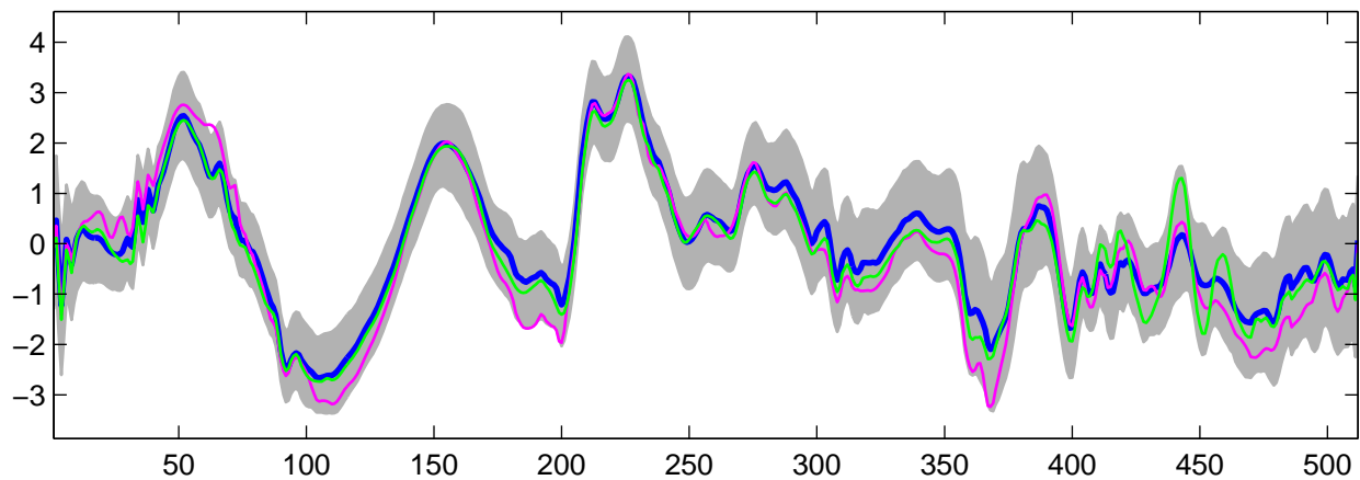
Estimated U_{31}(t) using G-WFMM: t_2 data, run 6
