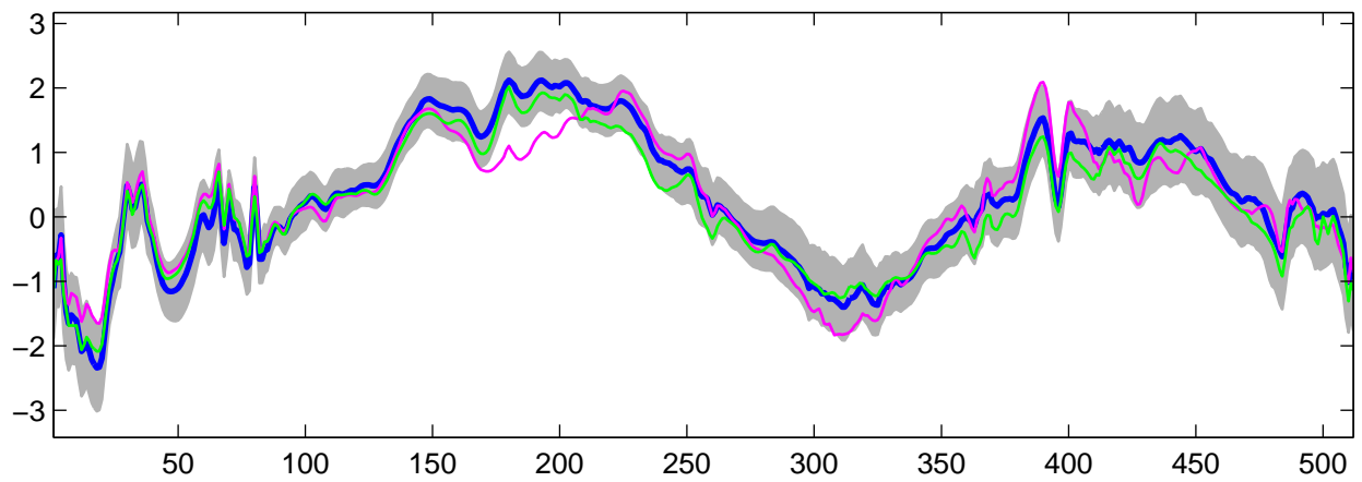
Estimated U_{31}(t) using R-WFMM: t_3 data, run 6
