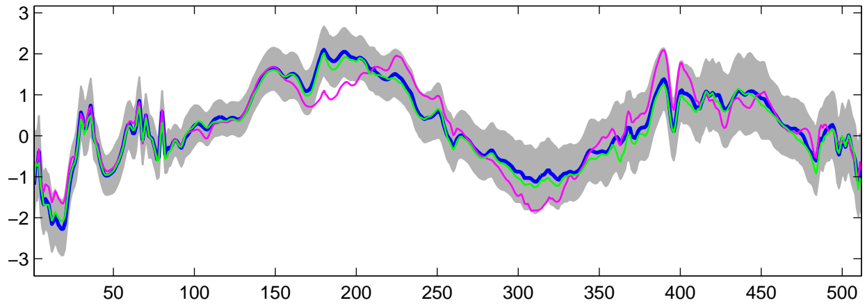
Estimated U_{31}(t) using G-WFMM: t_3 data, run 6
