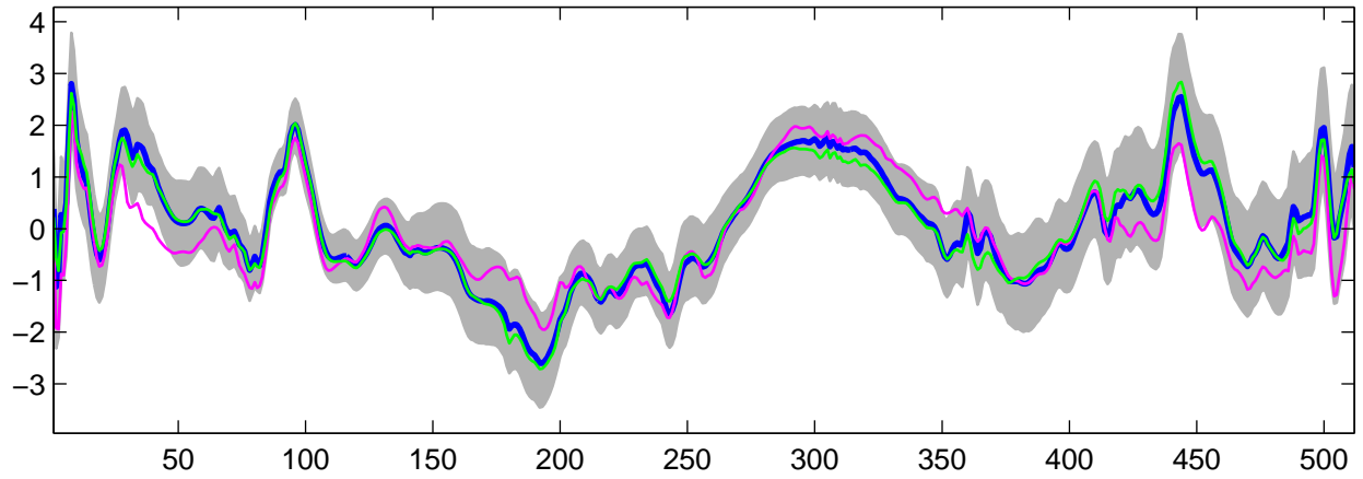
Estimated U_{32}(t) using G-WFMM: DE data, run 6
