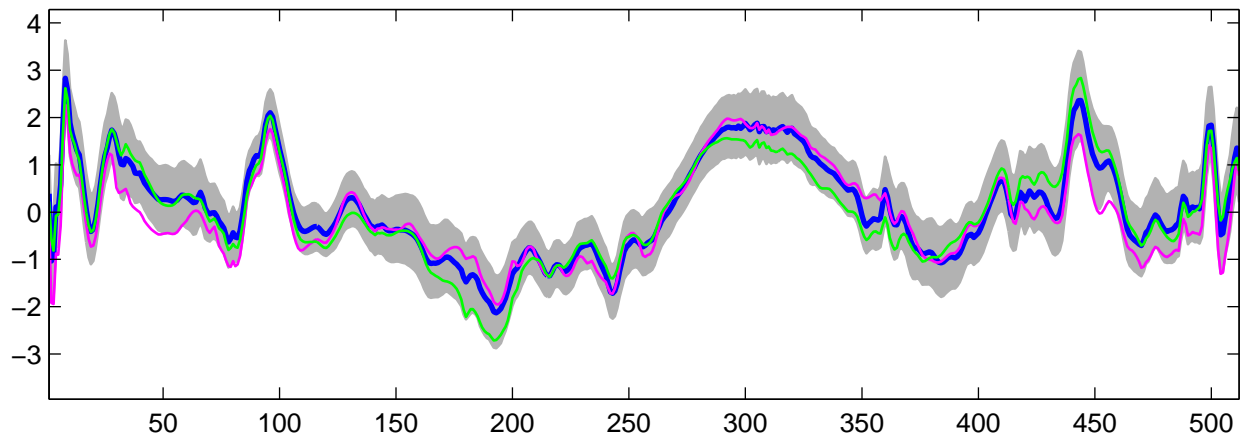
Estimated U_{32}(t) using R-WFMM: DE data, run 6
