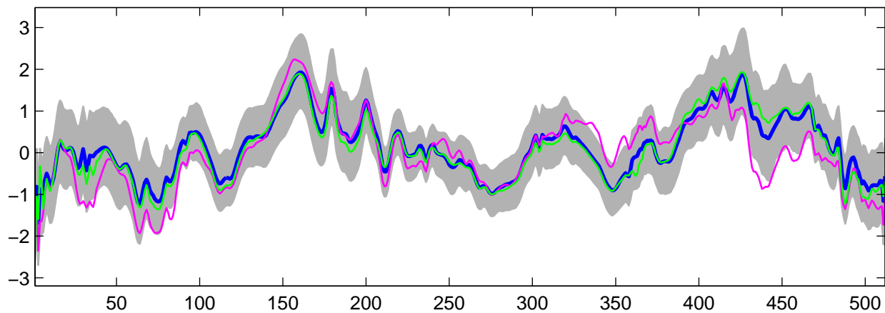
Estimated U_{32}(t) using G-WFMM: Normal data, run 6
