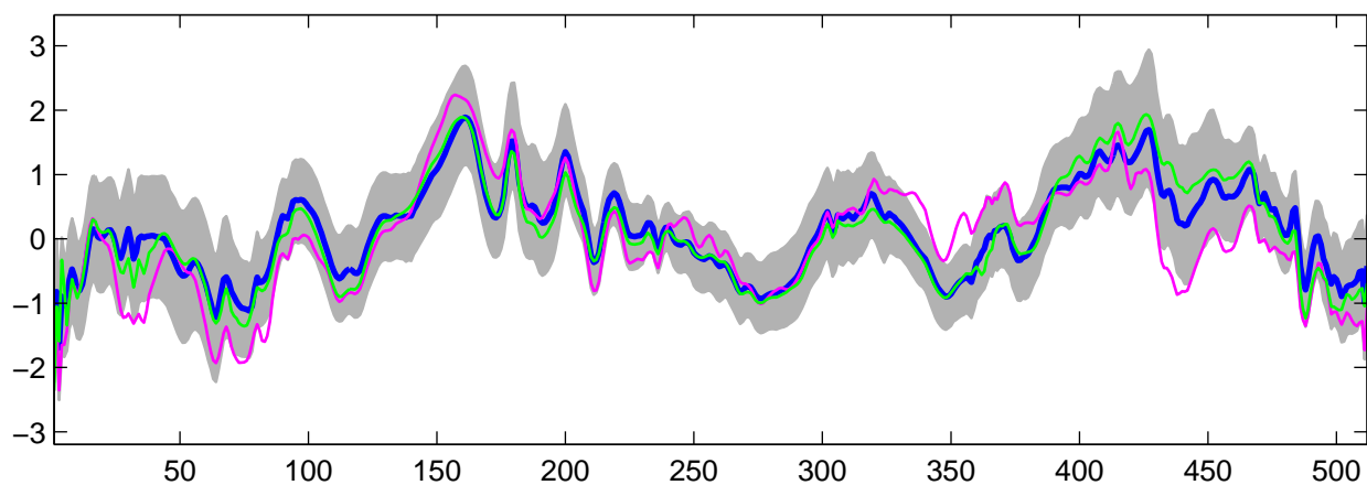
Estimated U_{32}(t) using R-WFMM: Normal data, run 6
