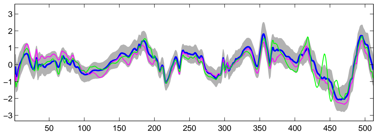
Estimated U_{32}(t) using R-WFMM: t_2 data, run 6
