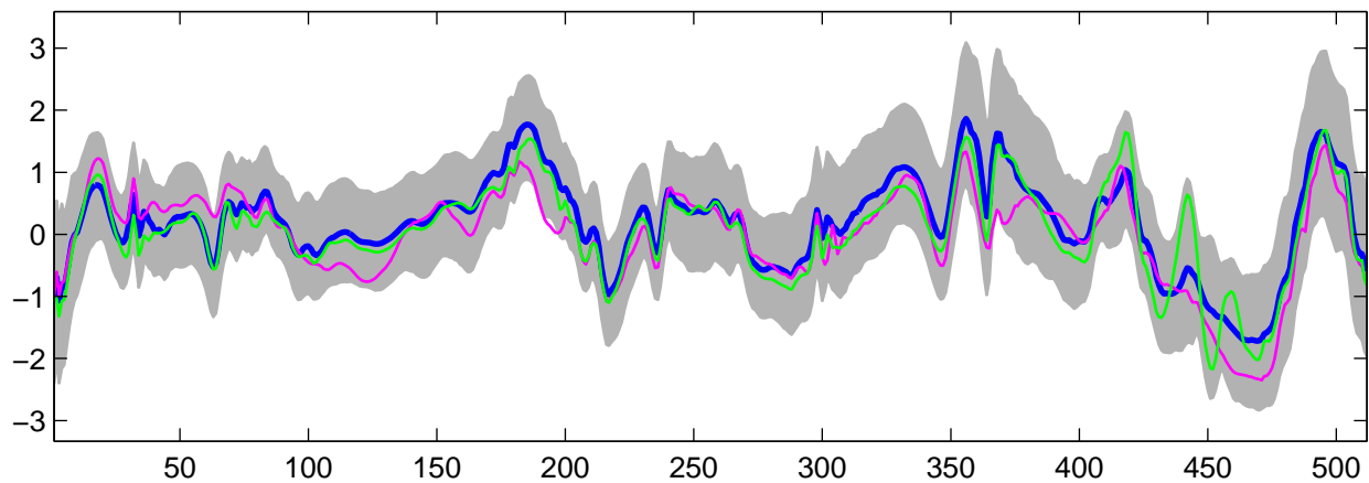
Estimated U_{32}(t) using G-WFMM: t_2 data, run 6
