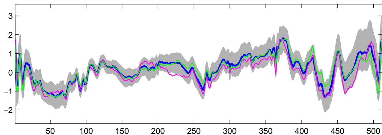
Estimated U_3(t) using R-WFMM: DE data, run 6
