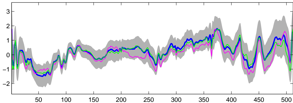
Estimated U_3(t) using G-WFMM: DE data, run 6
