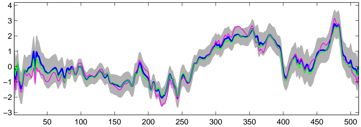
Estimated U_3(t) using G-WFMM: Normal data, run 6
