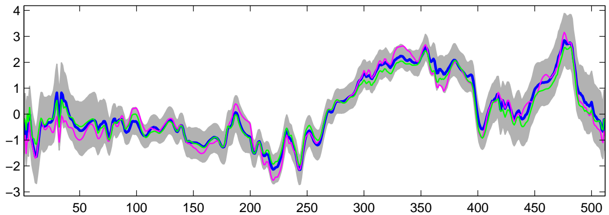
Estimated U_3(t) using R-WFMM: Normal data, run 6
