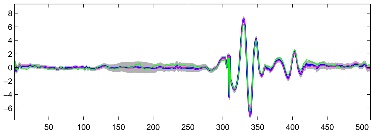
Estimated U_3(t) using R-WFMM: t_1 data, run 6
