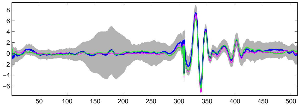
Estimated U_3(t) using G-WFMM: t_1 data, run 6
