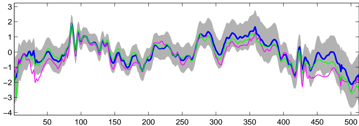
Estimated U_3(t) using G-WFMM: t_2 data, run 6
