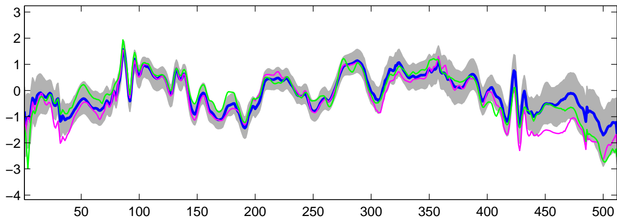
Estimated U_3(t) using R-WFMM: t_2 data, run 6
