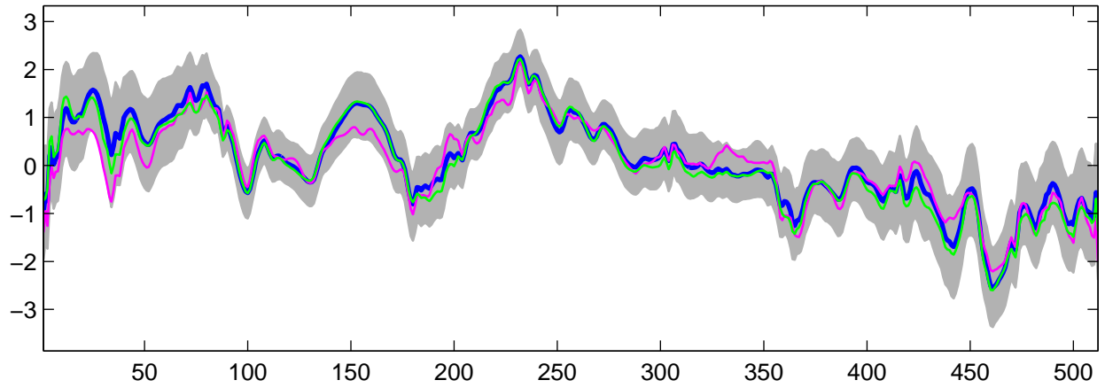
Estimated U_4(t) using G-WFMM: Normal data, run 6
