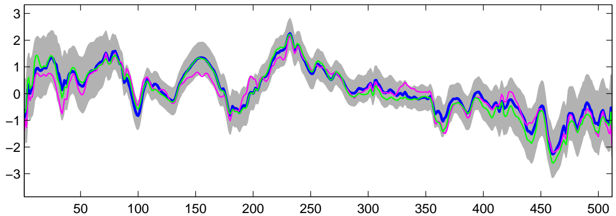
Estimated U_4(t) using R-WFMM: Normal data, run 6
