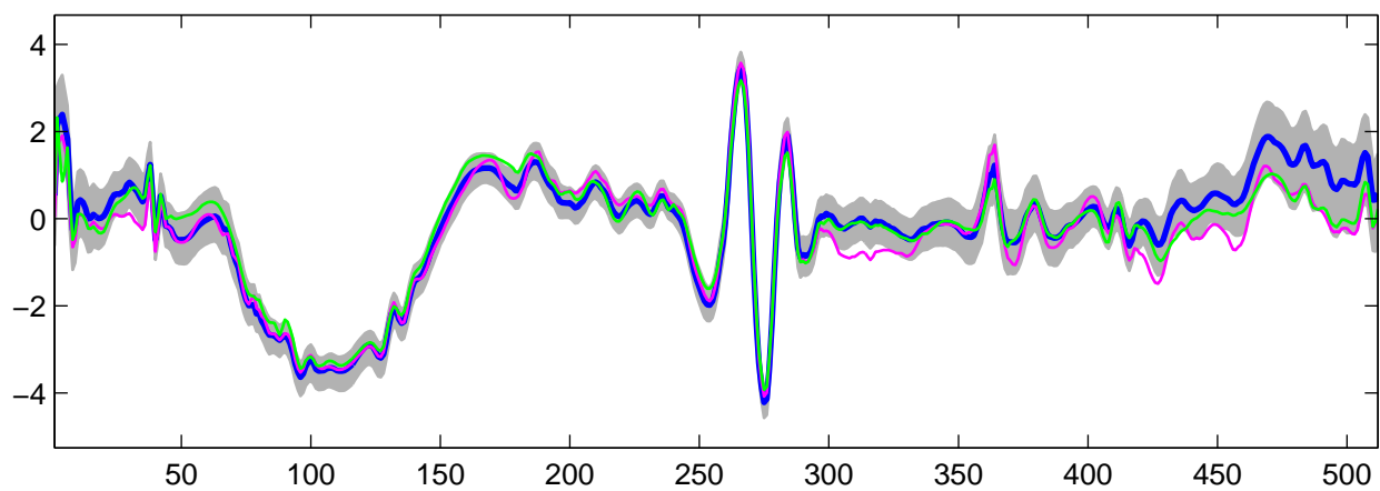
Estimated U_4(t) using R-WFMM: t_2 data, run 6
