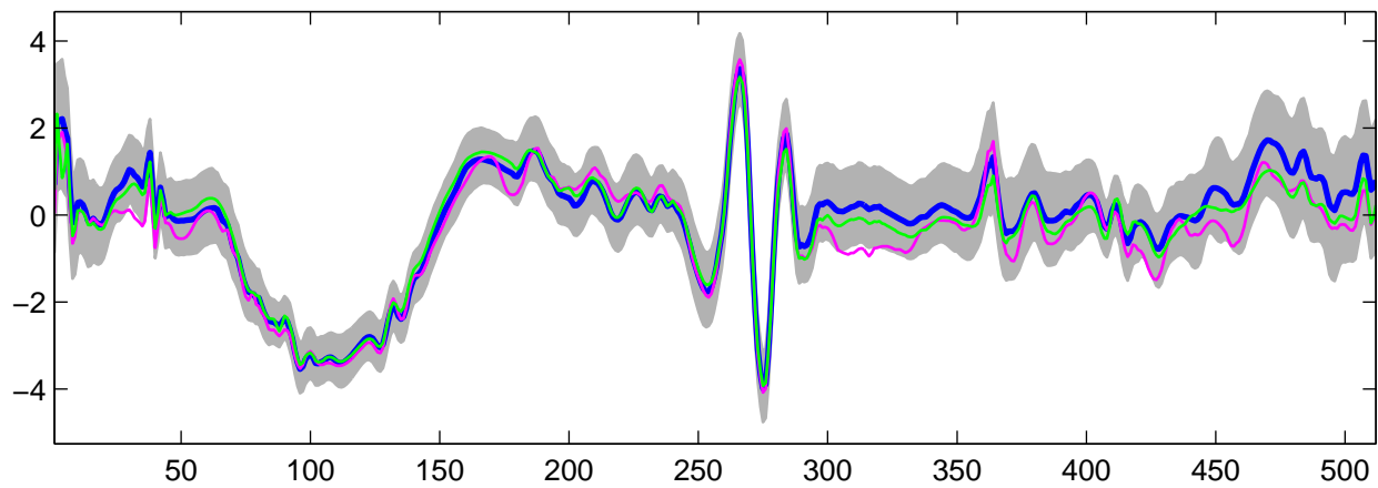
Estimated U_4(t) using G-WFMM: t_2 data, run 6
