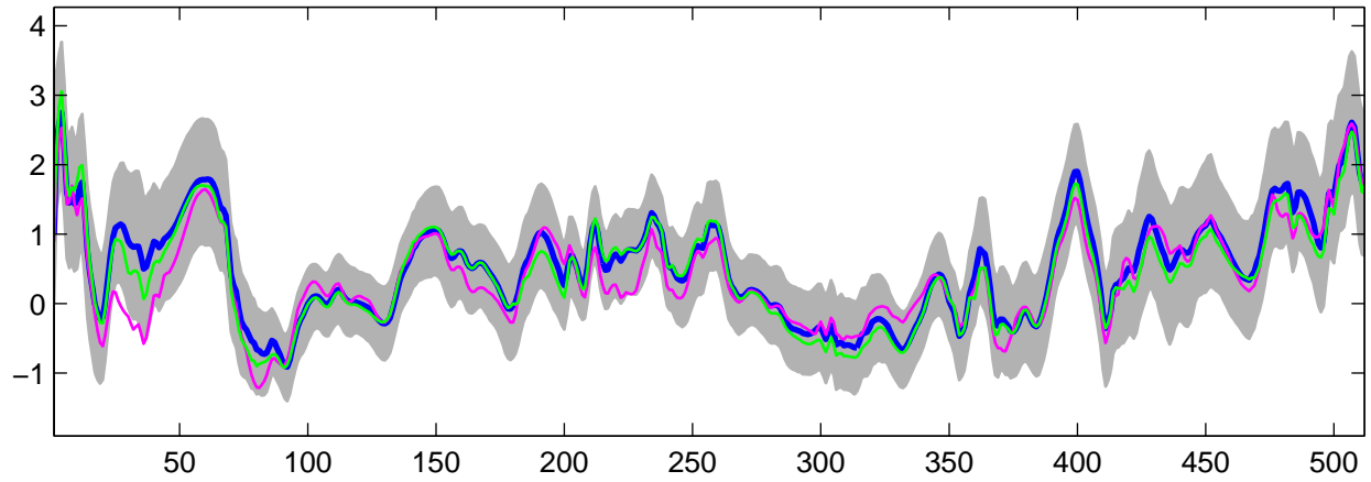
Estimated U_5(t) using G-WFMM: Normal data, run 6
