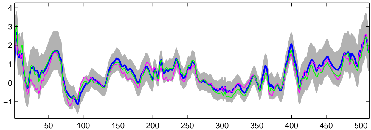
Estimated U_5(t) using R-WFMM: Normal data, run 6
