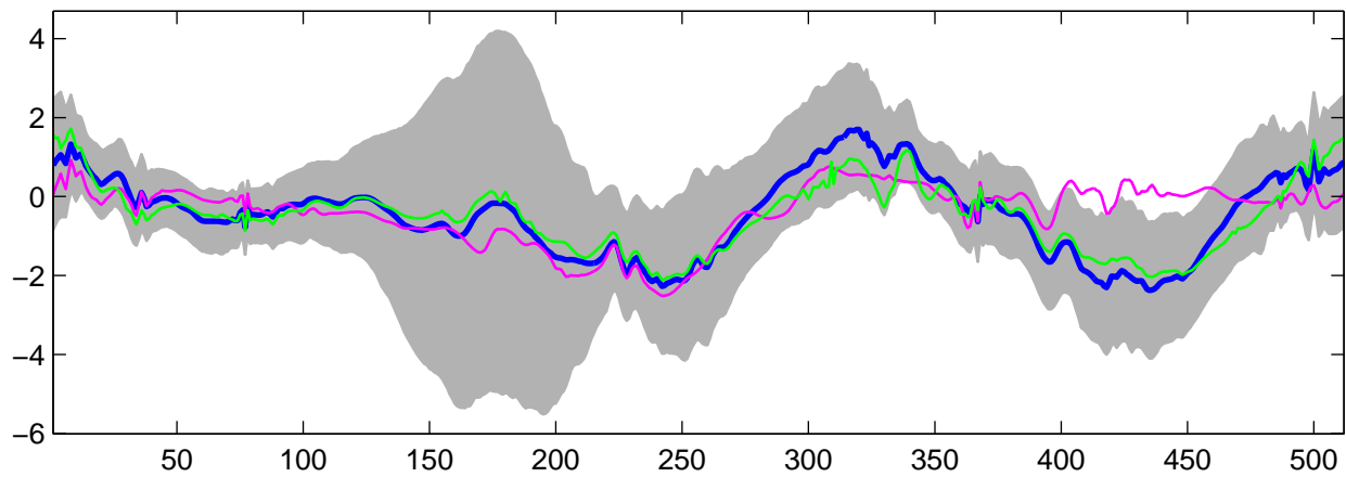
Estimated U_5(t) using G-WFMM: t_1 data, run 6
