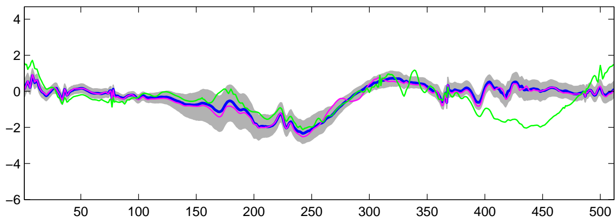
Estimated U_5(t) using R-WFMM: t_1 data, run 6
