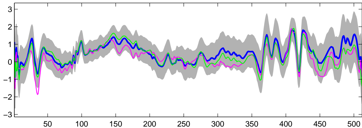
Estimated U_5(t) using G-WFMM: t_2 data, run 6
