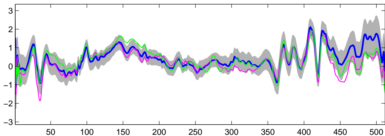
Estimated U_5(t) using R-WFMM: t_2 data, run 6
