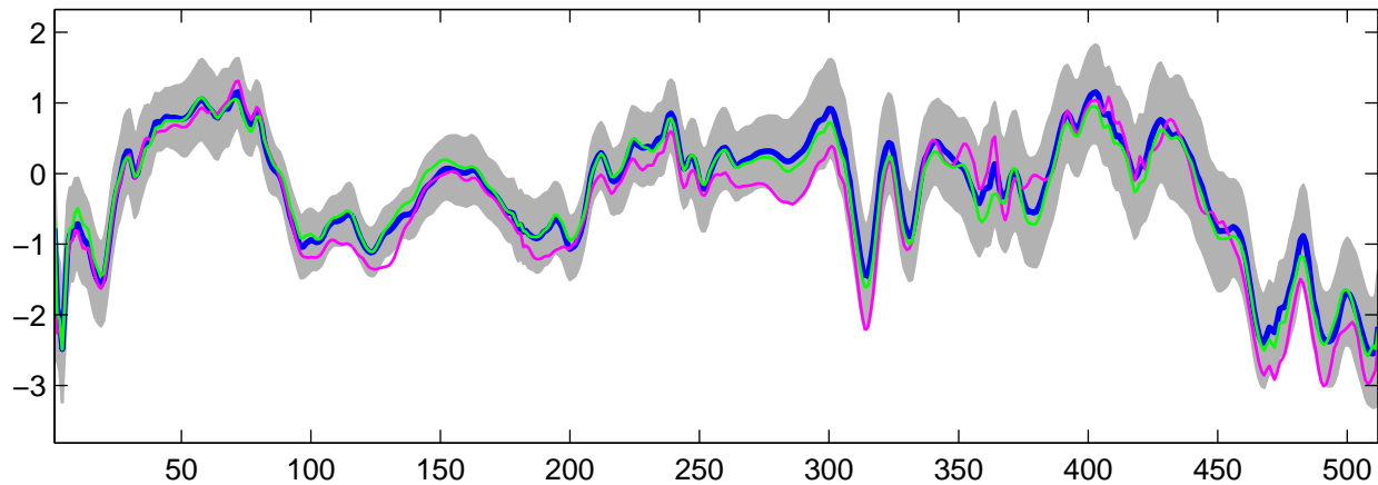
Estimated U_5(t) using G-WFMM: t_3 data, run 6
