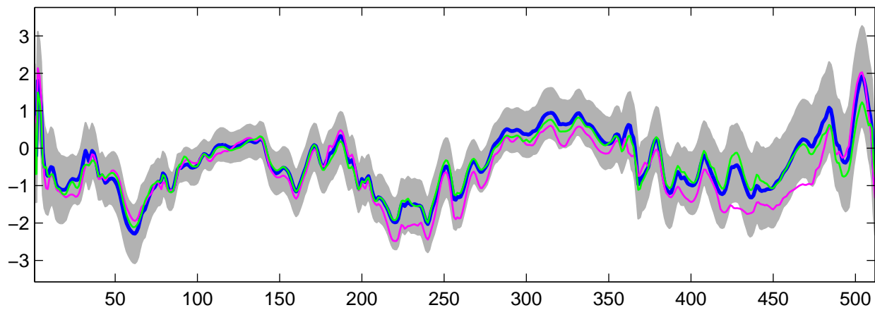
Estimated U_6(t) using G-WFMM: DE data, run 6
