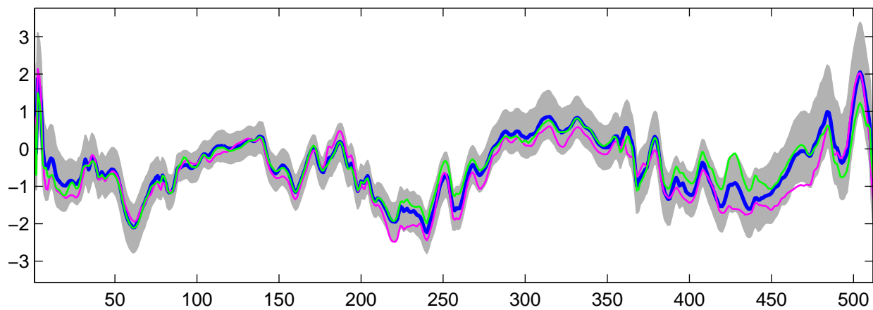
Estimated U_6(t) using R-WFMM: DE data, run 6
