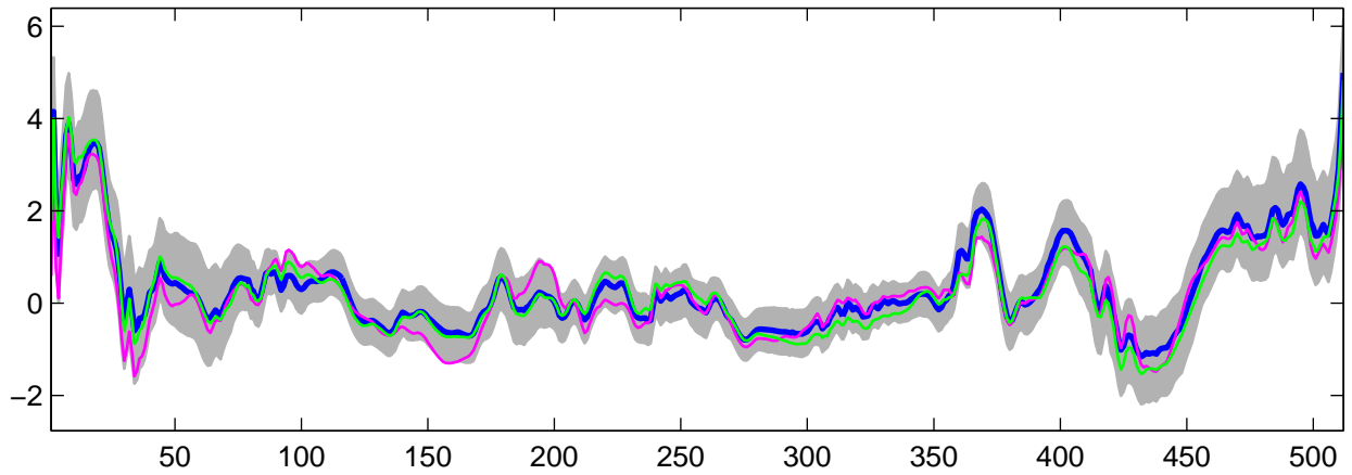
Estimated U_6(t) using R-WFMM: Normal data, run 6
