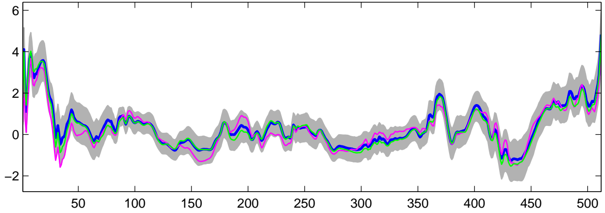
Estimated U_6(t) using G-WFMM: Normal data, run 6
