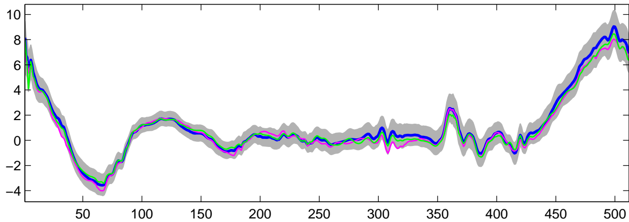
Estimated U_6(t) using G-WFMM: t_2 data, run 6
