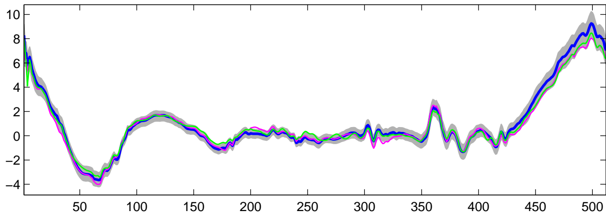
Estimated U_6(t) using R-WFMM: t_2 data, run 6
