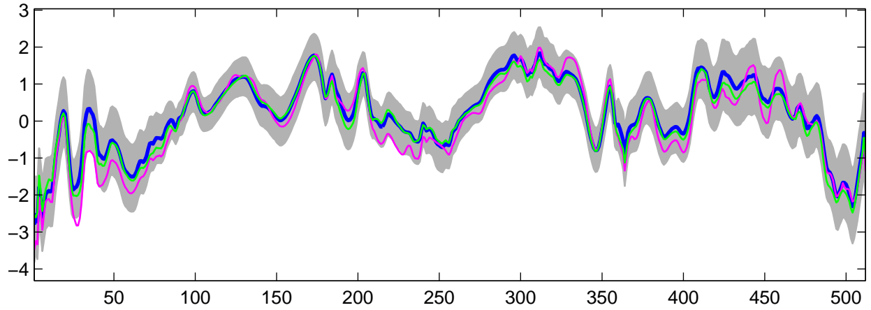
Estimated U_7(t) using G-WFMM: Normal data, run 6
