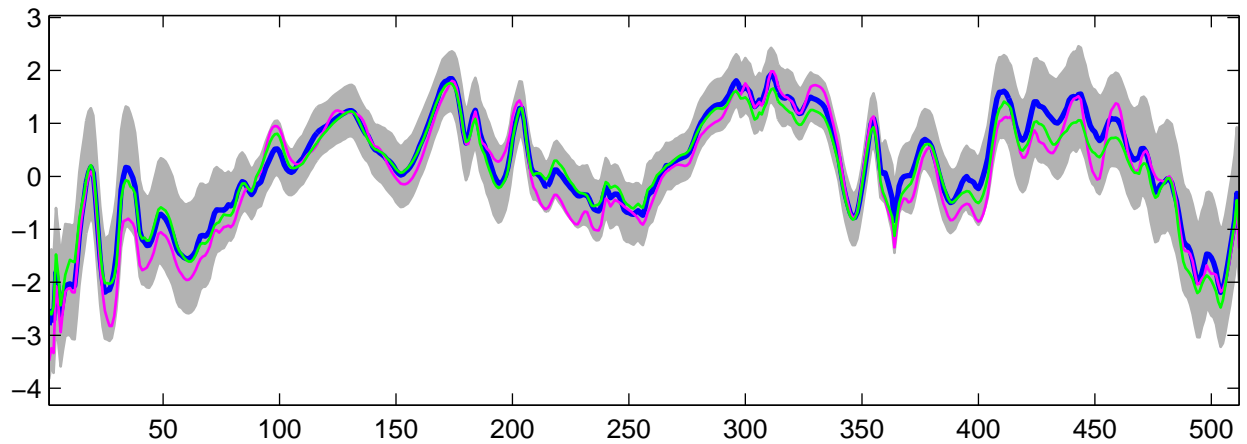
Estimated U_7(t) using R-WFMM: Normal data, run 6
