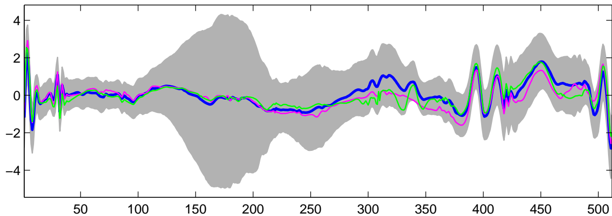
Estimated U_7(t) using G-WFMM: t_1 data, run 6
