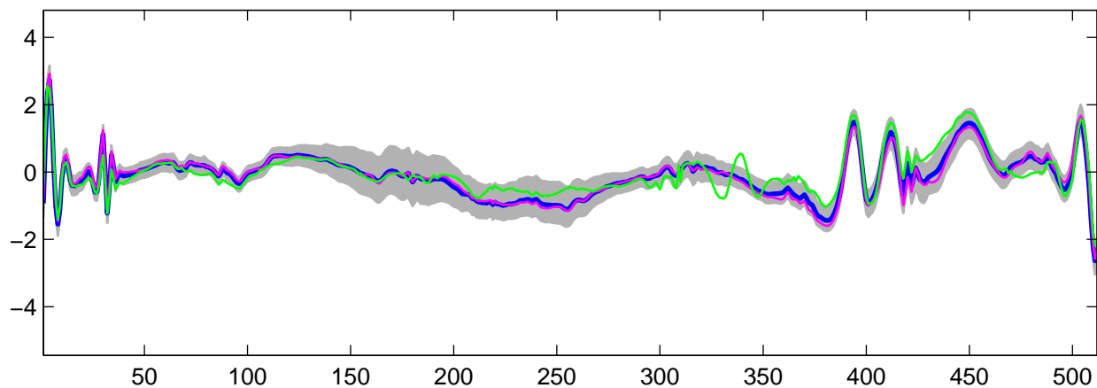
Estimated U_7(t) using R-WFMM: t_1 data, run 6
