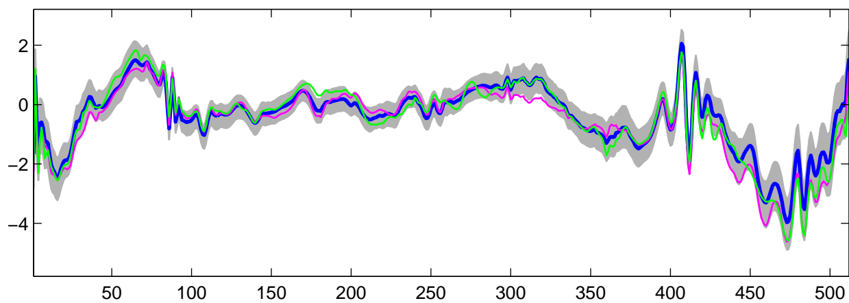
Estimated U_7(t) using R-WFMM: t_2 data, run 6
