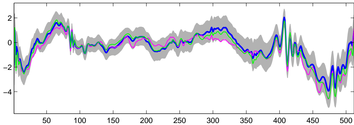
Estimated U_7(t) using G-WFMM: t_2 data, run 6
