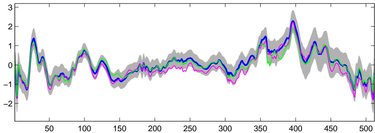
Estimated U_7(t) using R-WFMM: t_3 data, run 6
