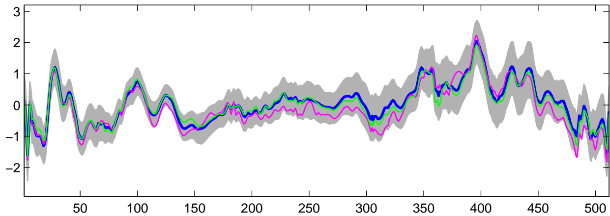
Estimated U_7(t) using G-WFMM: t_3 data, run 6
