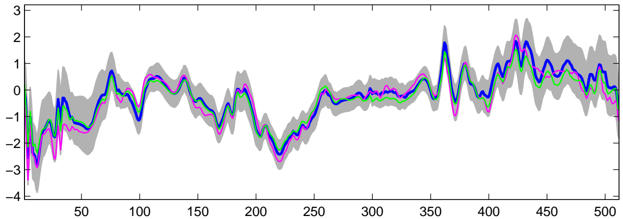
Estimated U_g(t) using R-WFMM: Normal data, run 6
