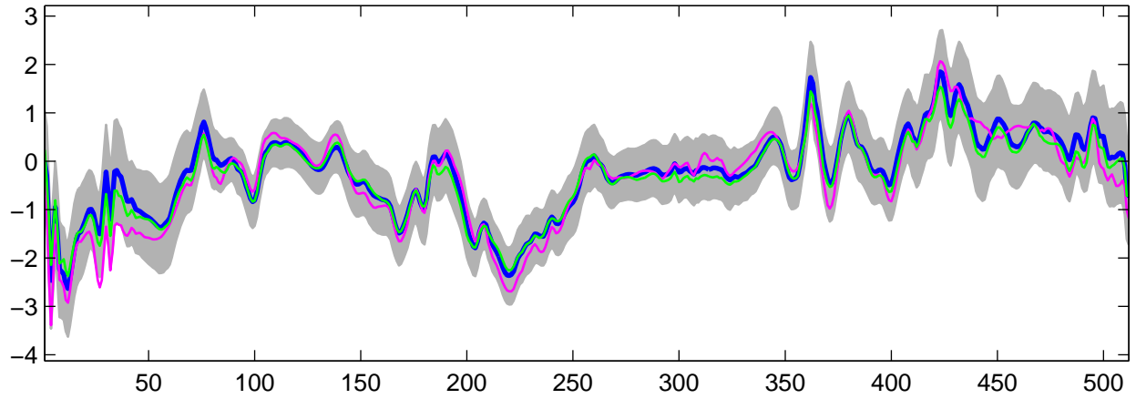
Estimated U_g(t) using G-WFMM: Normal data, run 6
