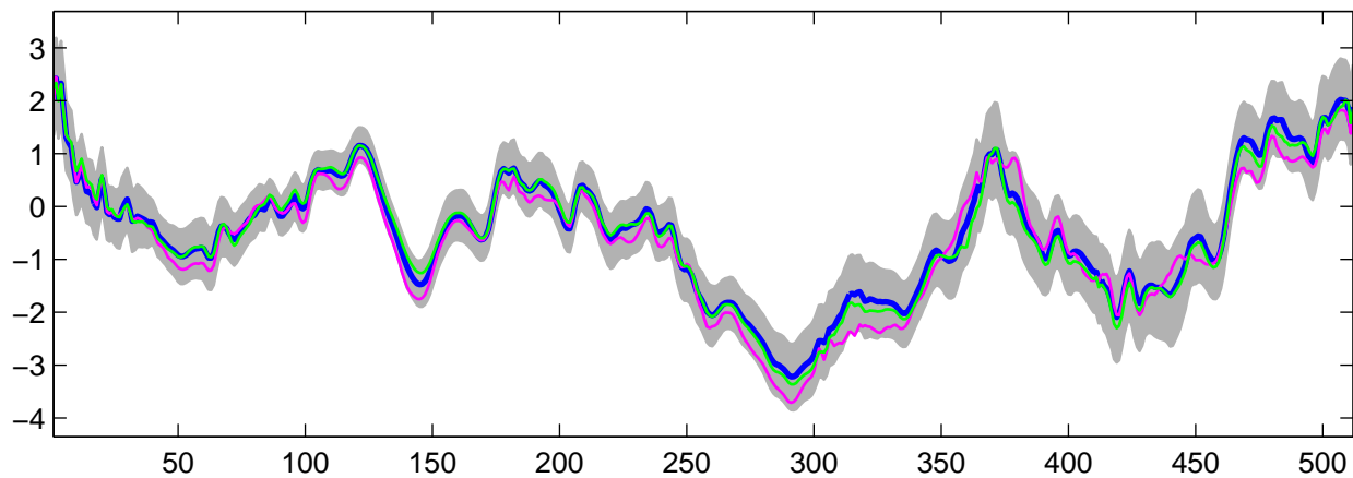
Estimated U_8(t) using G-WFMM: t_3 data, run 6
