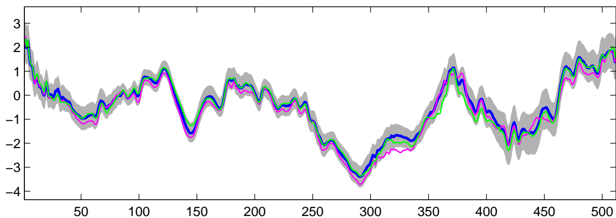
Estimated U_8(t) using R-WFMM: t_3 data, run 6
