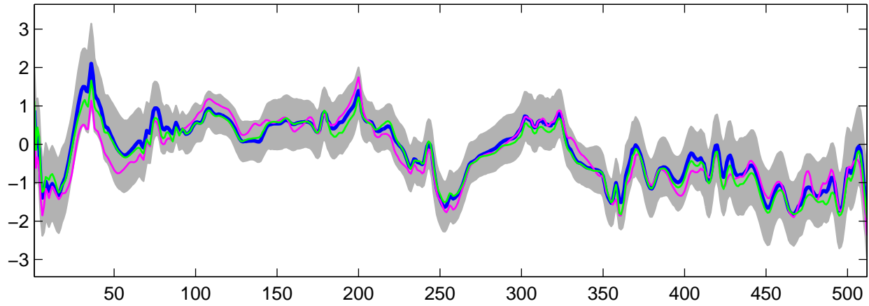
Estimated U_{\theta}(t) using G-WFMM: Normal data, run 6
