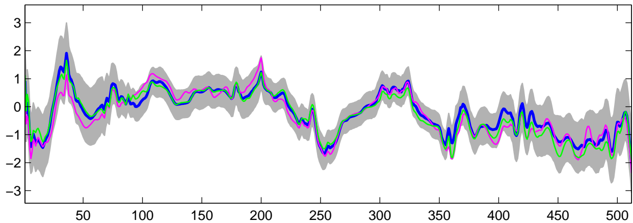
Estimated U_{\theta}(t) using R-WFMM: Normal data, run 6
