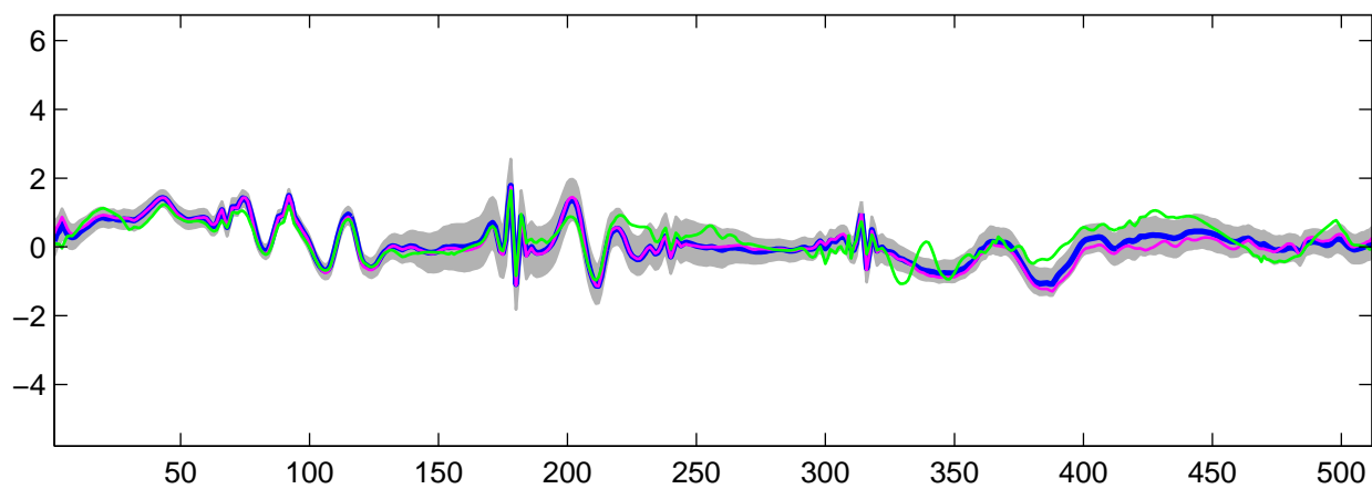
Estimated U_{\theta}(t) using R-WFMM: t_1 data, run 6
