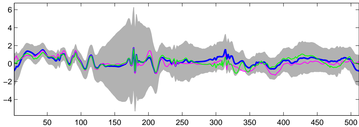
Estimated U_{\theta}(t) using G-WFMM: t_1 data, run 6
