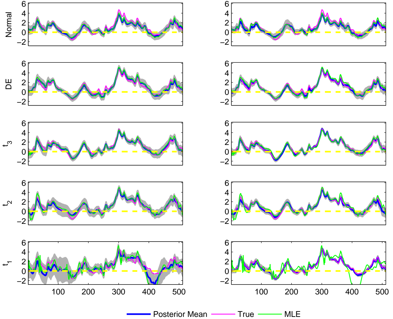
The estimated B_2(t) for 5 simulated datasets, simulation run 7
