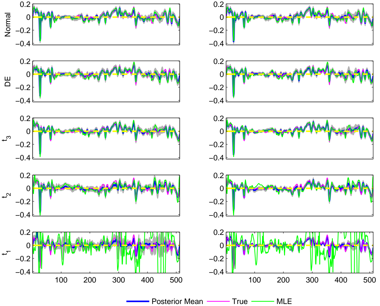
The estimated B_5(t) for 5 simulated datasets, simulation run 7
