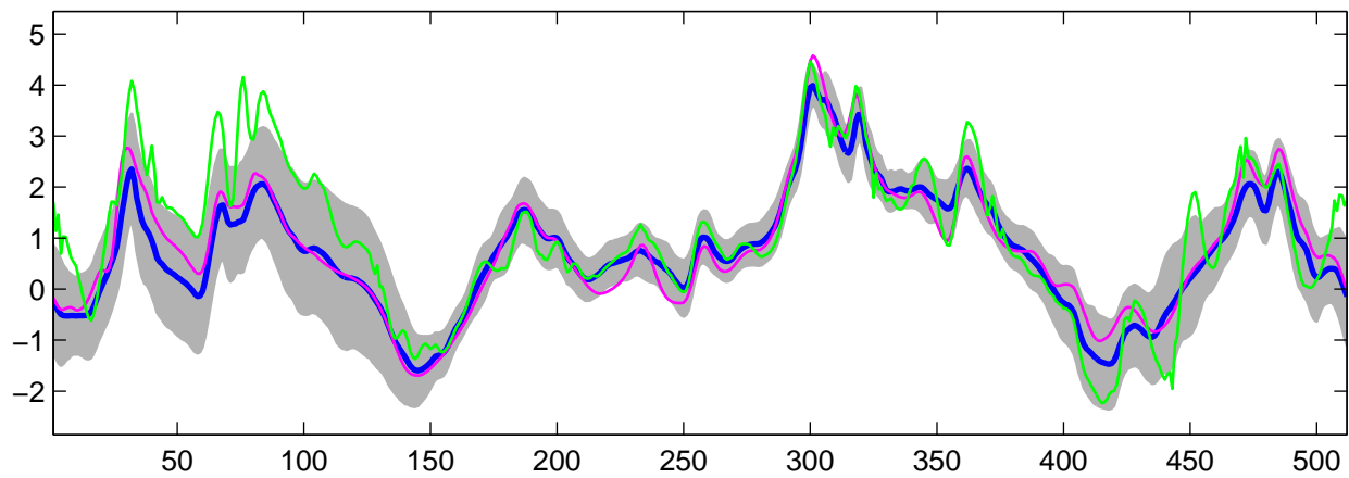
Estimated C_0(t) using G-WFMM: t_1 data, run 7
