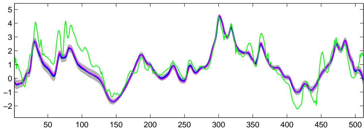
Estimated C_0(t) using R-WFMM: t_1 data, run 7
