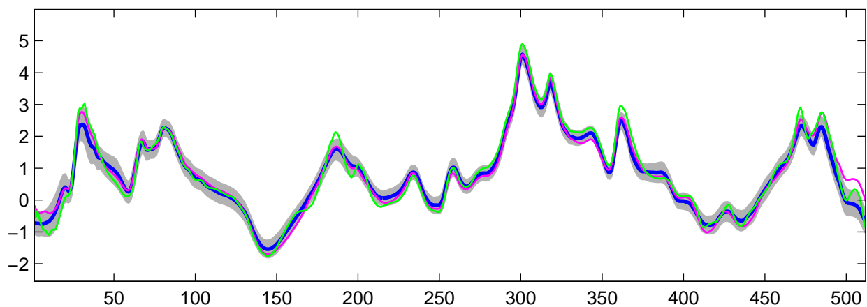
Estimated C_0(t) using R-WFMM: t_2 data, run 7
