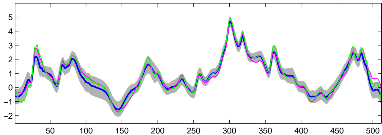
Estimated C_0(t) using G-WFMM: t_2 data, run 7
