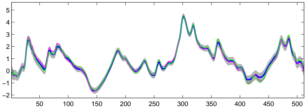
Estimated C_0(t) using R-WFMM: t_3 data, run 7
