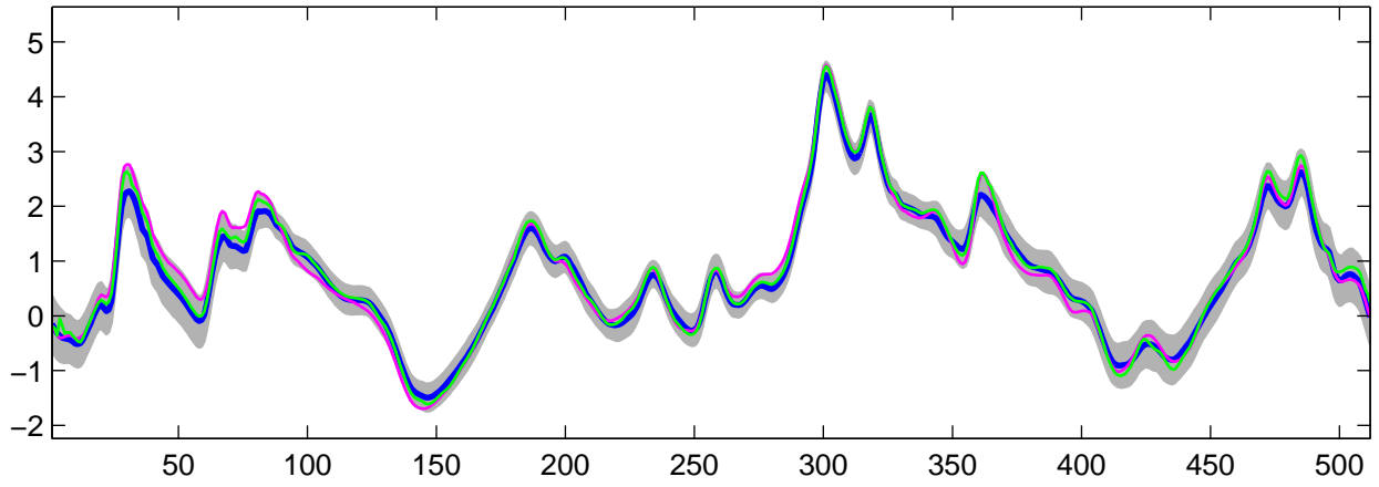
Estimated C_0(t) using G-WFMM: t_3 data, run 7
