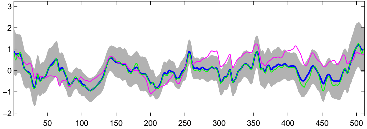
Estimated C_1(t) using G-WFMM: Normal data, run 7
