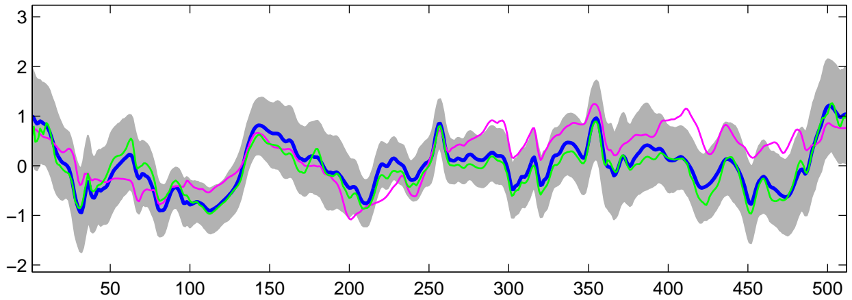
Estimated C_1(t) using R-WFMM: Normal data, run 7
