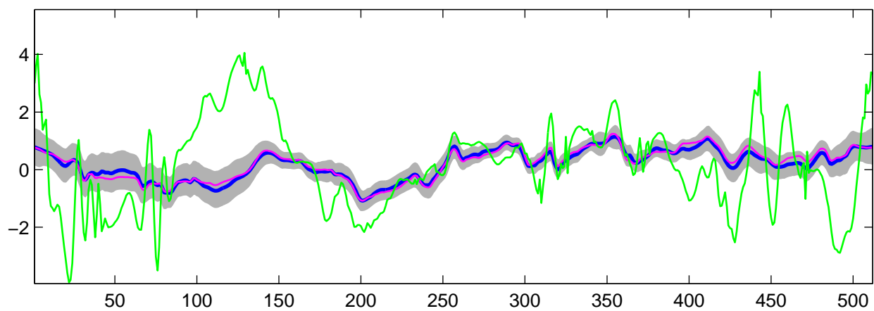
Estimated C_1(t) using R-WFMM: t_1 data, run 7
