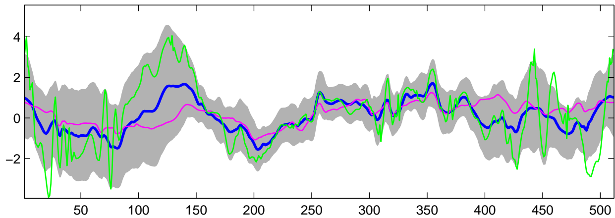
Estimated C_1(t) using G-WFMM: t_1 data, run 7
