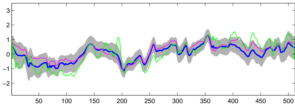
Estimated C_1(t) using R-WFMM: t_2 data, run 7
