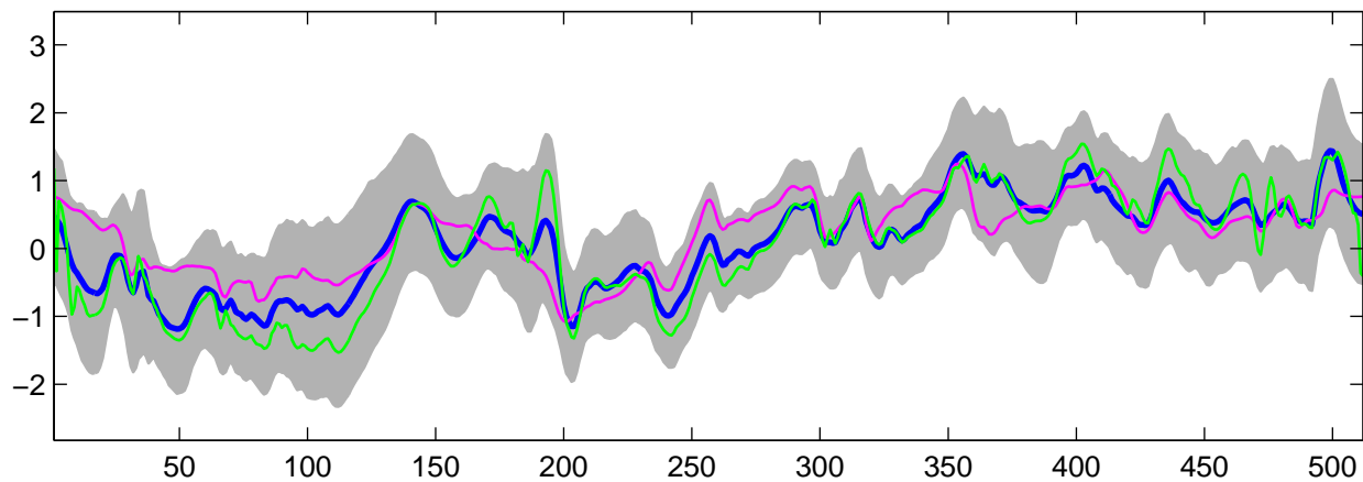
Estimated C_1(t) using G-WFMM: t_2 data, run 7
