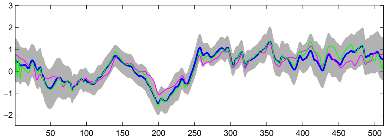
Estimated C_1(t) using G-WFMM: t_3 data, run 7
