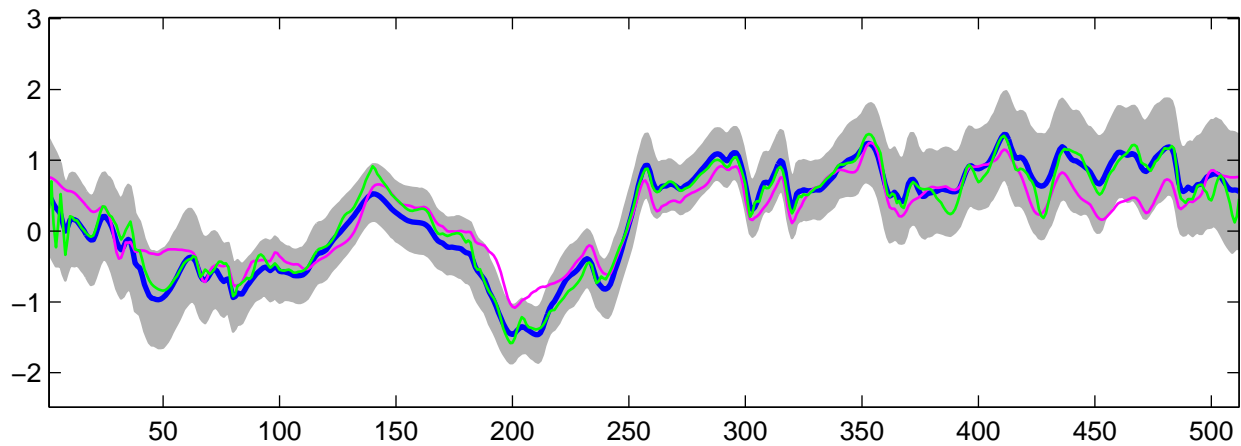
Estimated C_1(t) using R-WFMM: t_3 data, run 7
