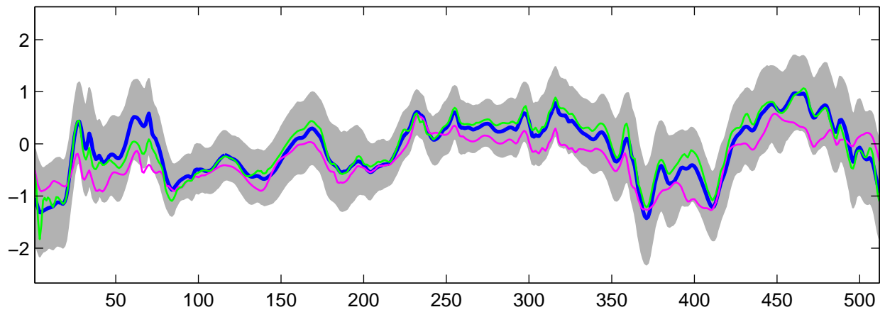
Estimated C_2(t) using R-WFMM: Normal data, run 7
