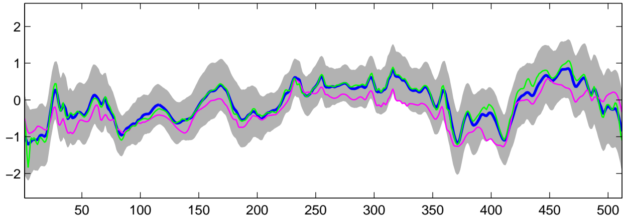
Estimated C_2(t) using G-WFMM: Normal data, run 7
