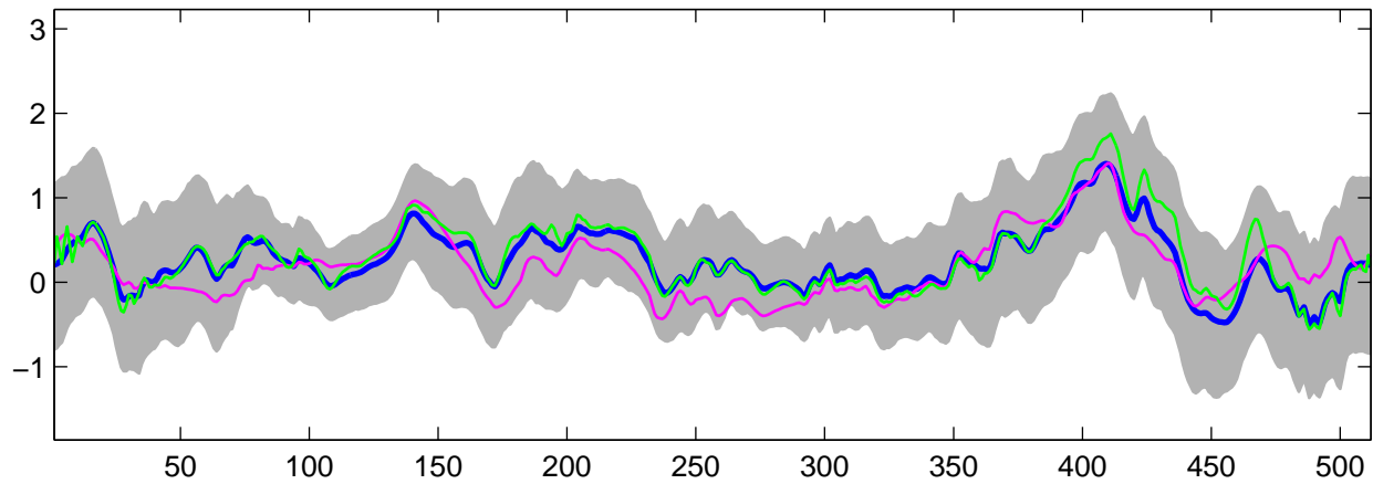
Estimated C_3(t) using G-WFMM: DE data, run 7
