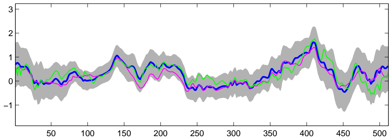
Estimated C_3(t) using R-WFMM: DE data, run 7
