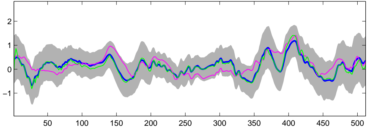
Estimated C_3(t) using G-WFMM: Normal data, run 7
