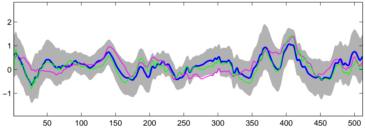
Estimated C_3(t) using R-WFMM: Normal data, run 7
