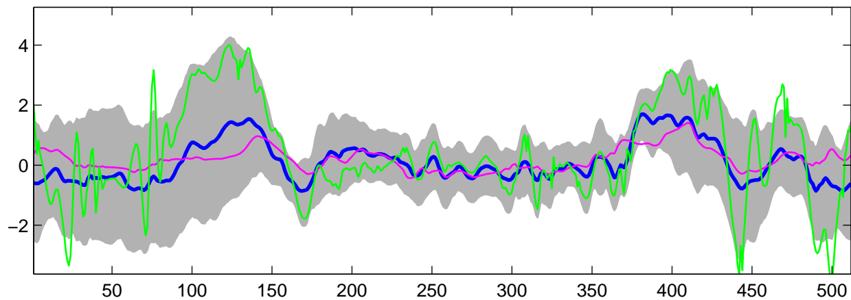
Estimated C_3(t) using G-WFMM: t_1 data, run 7
