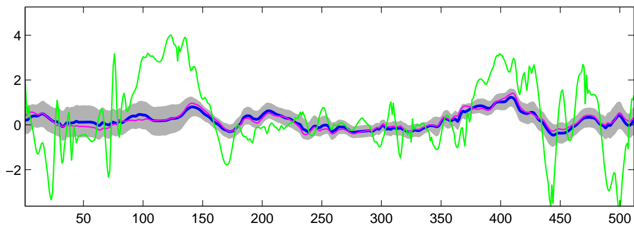
Estimated C_3(t) using R-WFMM: t_1 data, run 7
