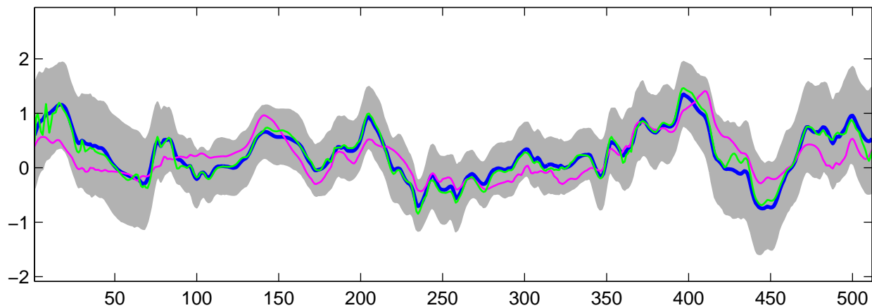
Estimated C_3(t) using G-WFMM: t_3 data, run 7
