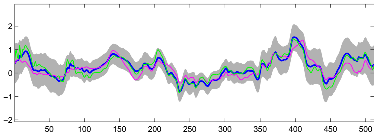
Estimated C_3(t) using R-WFMM: t_3 data, run 7
