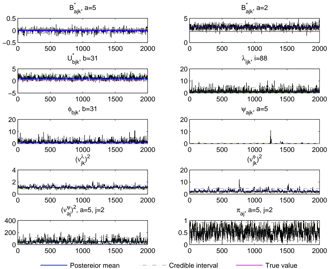
Trace plot, j=2, k=6 , DE data, simulation run 7
