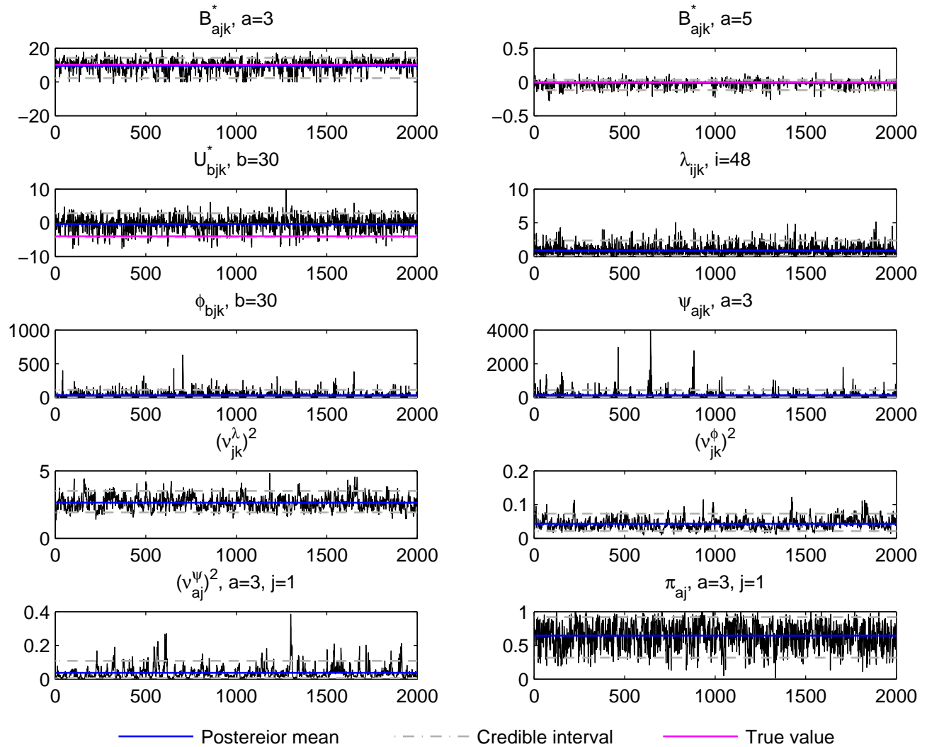
Trace plot, j=1, k=5 , Normal data, simulation run 7
