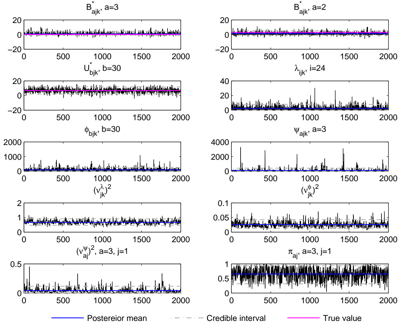
Trace plot, j=1, k=6, t_2 data, simulation run 7
