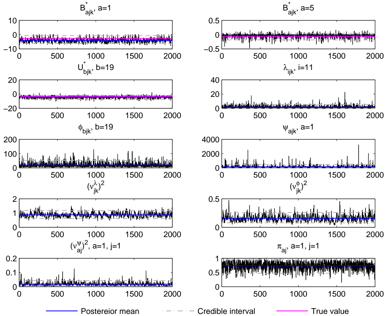
Trace plot, j=1, k=8, t_3 data, simulation run 7
