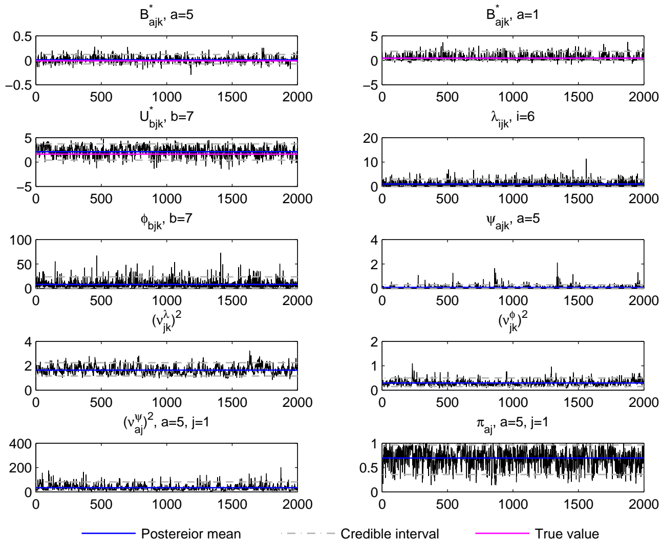
Trace plot, j=1, k=6 , DE data, simulation run 7
