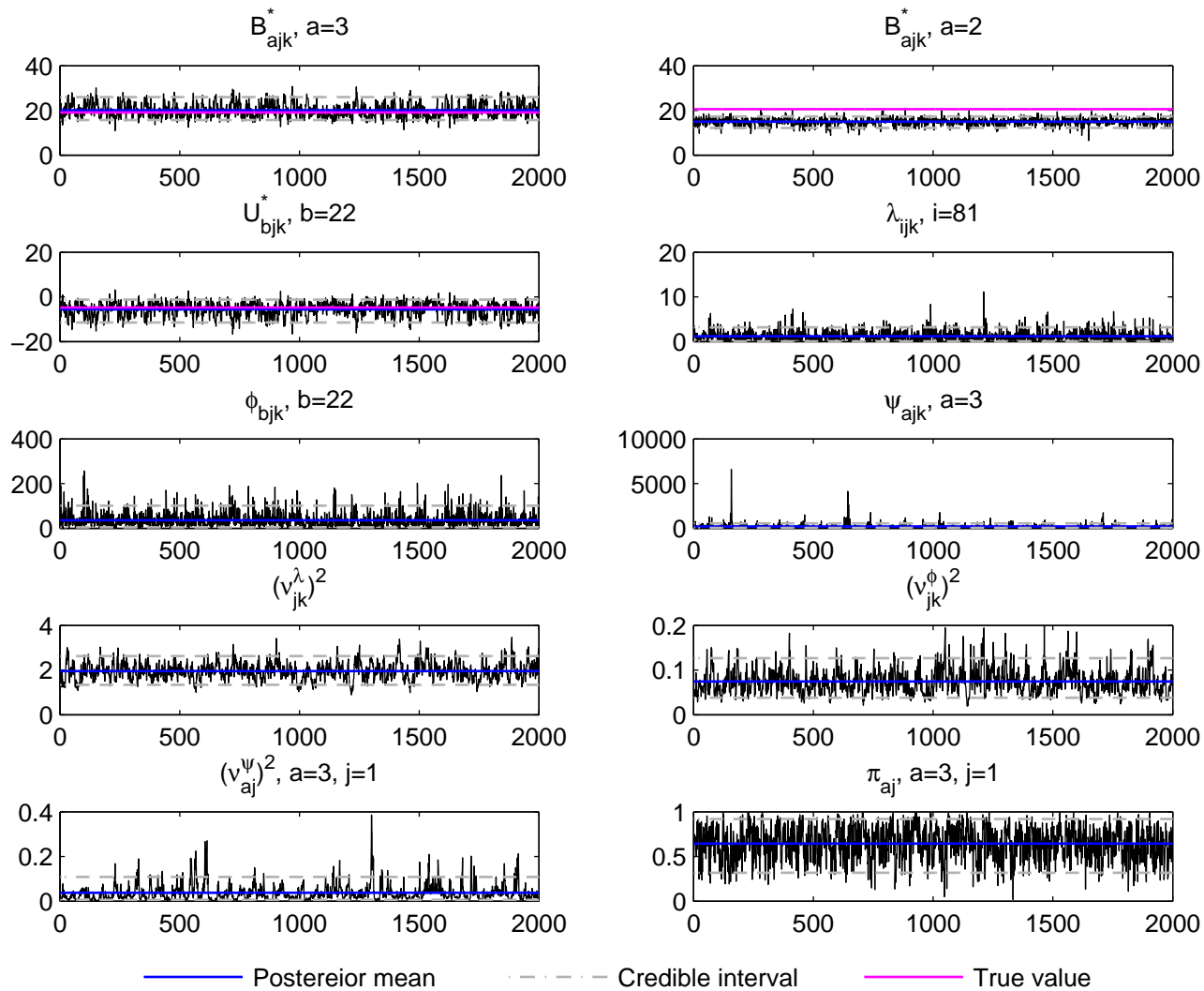
Trace plot, j=1, k=1 , Normal data, simulation run 7
