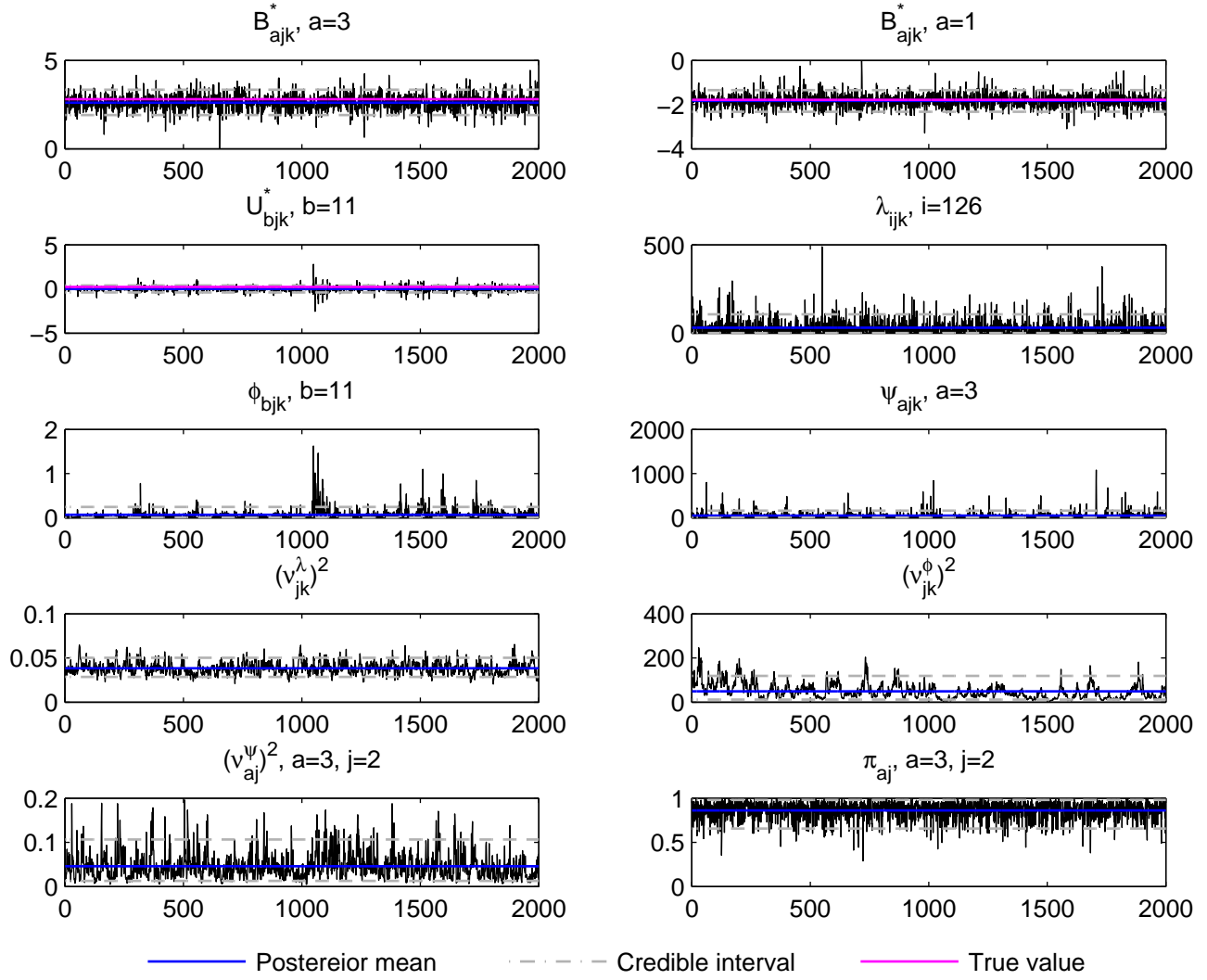
Trace plot, j=2, k=7, t_j data, simulation run 7
