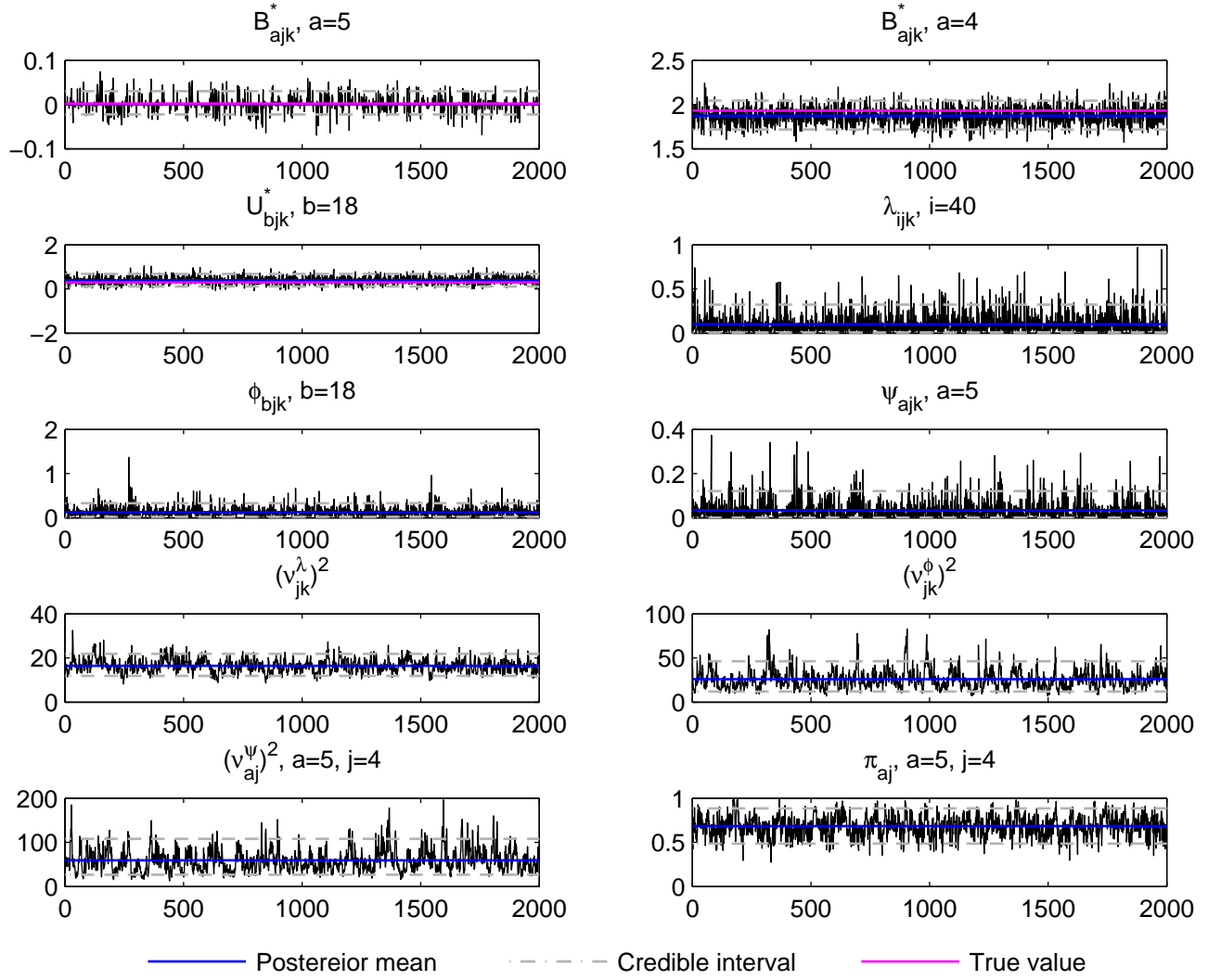
Trace plot, j=4, k=4, t_2 data, simulation run 7
